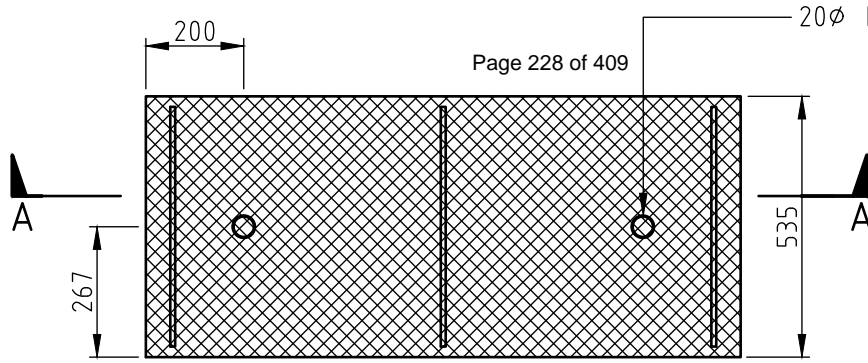
PLAN OF 6mm CHEQUER PLATE
