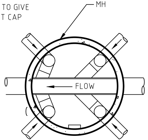
GENERAL APPROACH POSITION RELATED TO MANHOLE 1 ONLY IN MANHOLE
