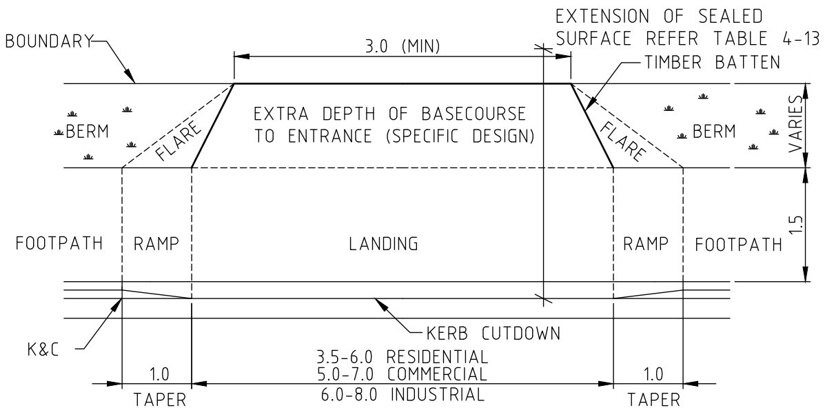
VEHICLE ENTRANCE PLAN
