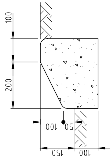
MOUNTABLE KERB
