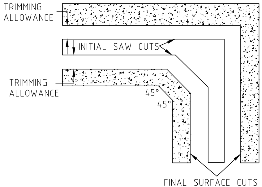
FIG 3 - TRENCH EXCAVATION WITH CORNERS PLAN VIEW
